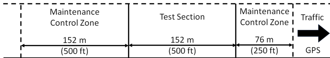
Figure 10. LTPP GPS Test Section General Layout (Elkins and Ostrom, 2021).
