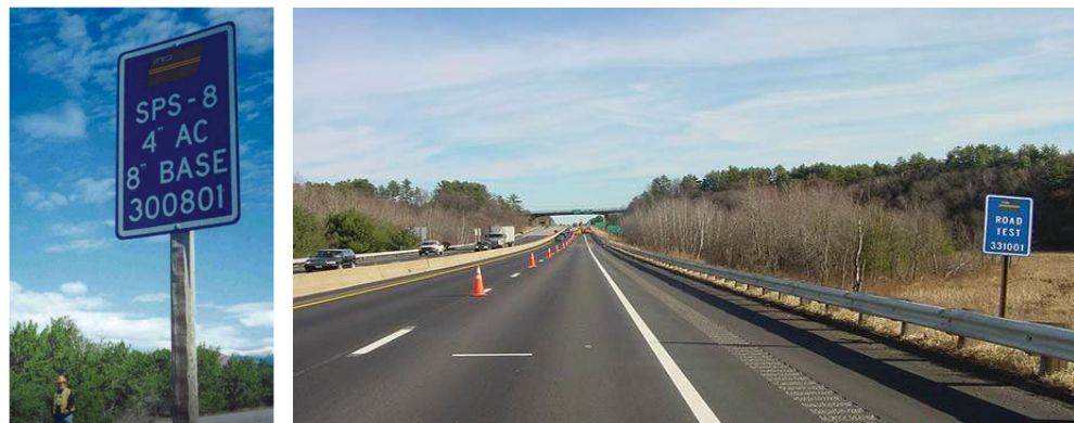
Figure 12. Examples of SHRP/LTPP Test Section Road Signs.
